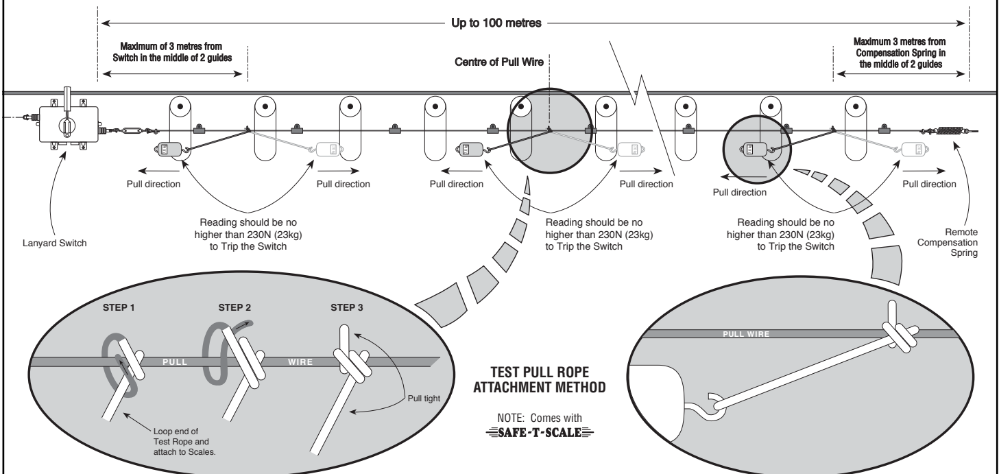
FIGURE 1 Axis Pull Wire Test
