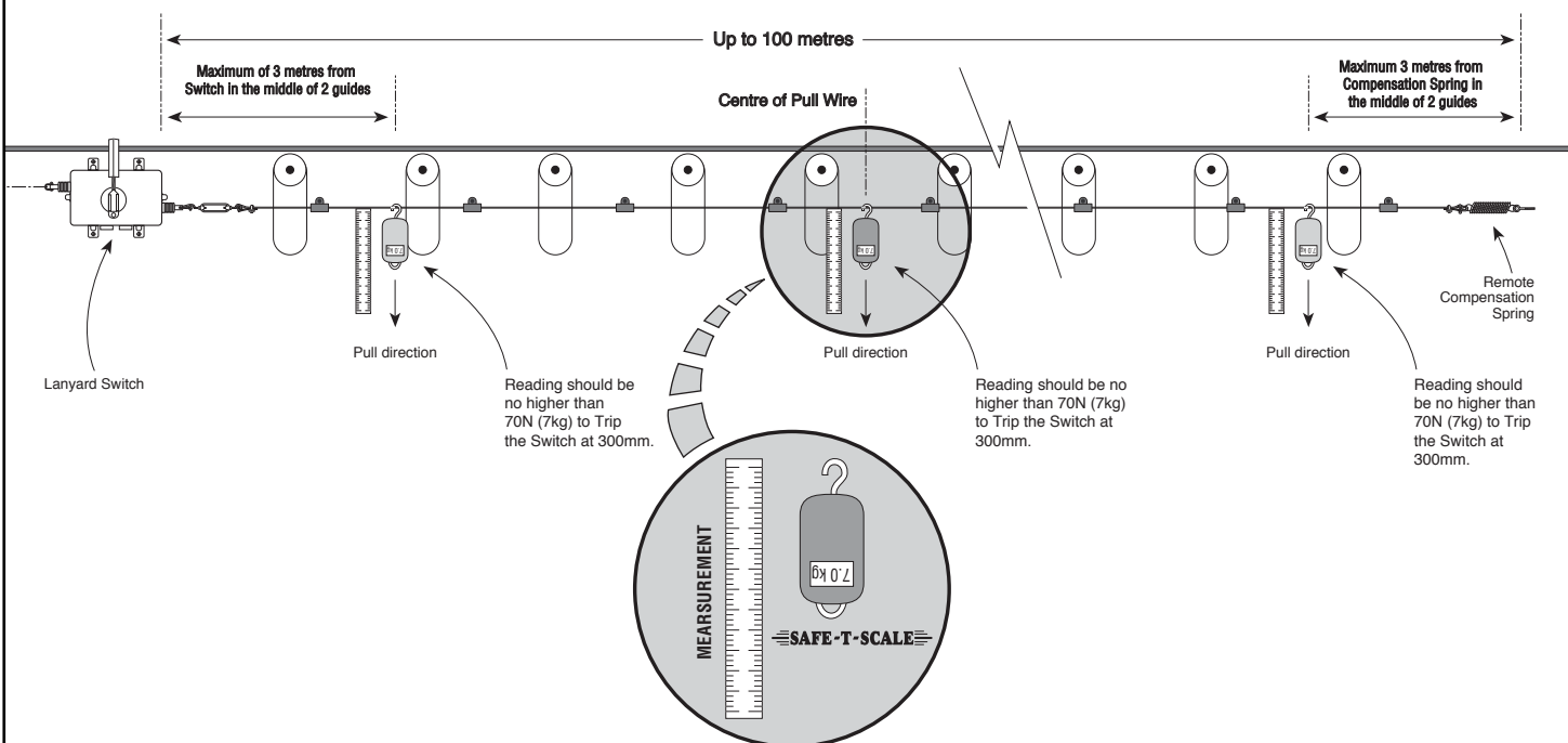
FIGURE 2 90 Degree Pull Wire Test
